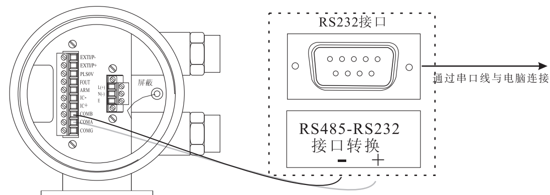
B、RS485接线
