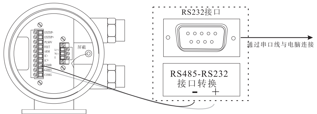
B、RS485接线
