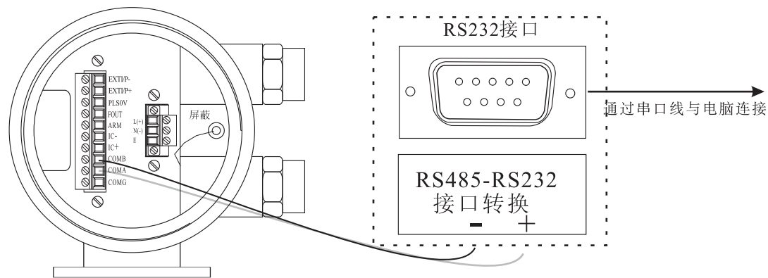
B、RS485接线
