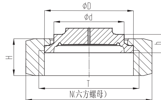
RJT-BS4825-5 槽型螺母
